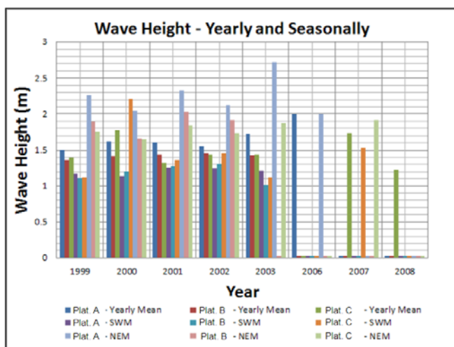
Fig. 5 Wave Height – Yearly and Seasonally For Platform A, Platform B and Platform C
