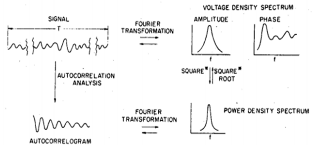
Fig. 1 Relationships between a signal and its analyses
