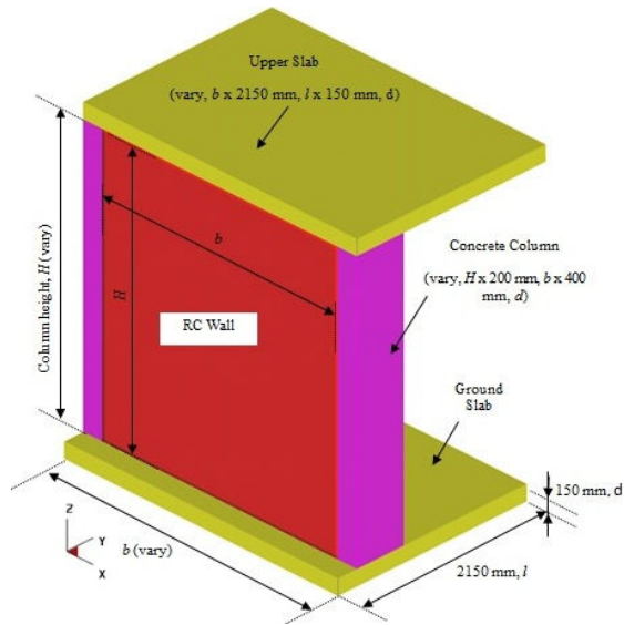
Fig. 3 Dimension details of RC wall
