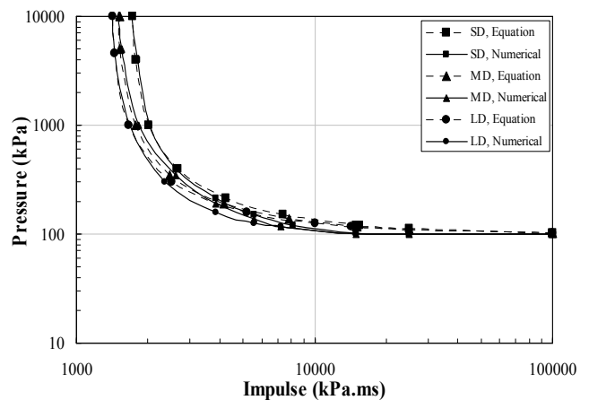
Fig. 4 P-I curves of one-way panel P1
