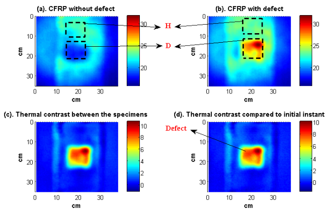
Fig. 7 Thermograms at the instant 41 s
