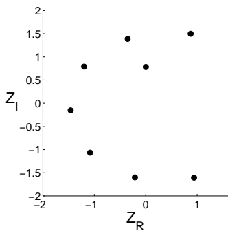
Fig. 3. The distributions of zeros in table.(IV).
