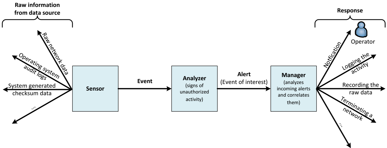
Fig. 1. Components of an Intrusion Detection System [4]
