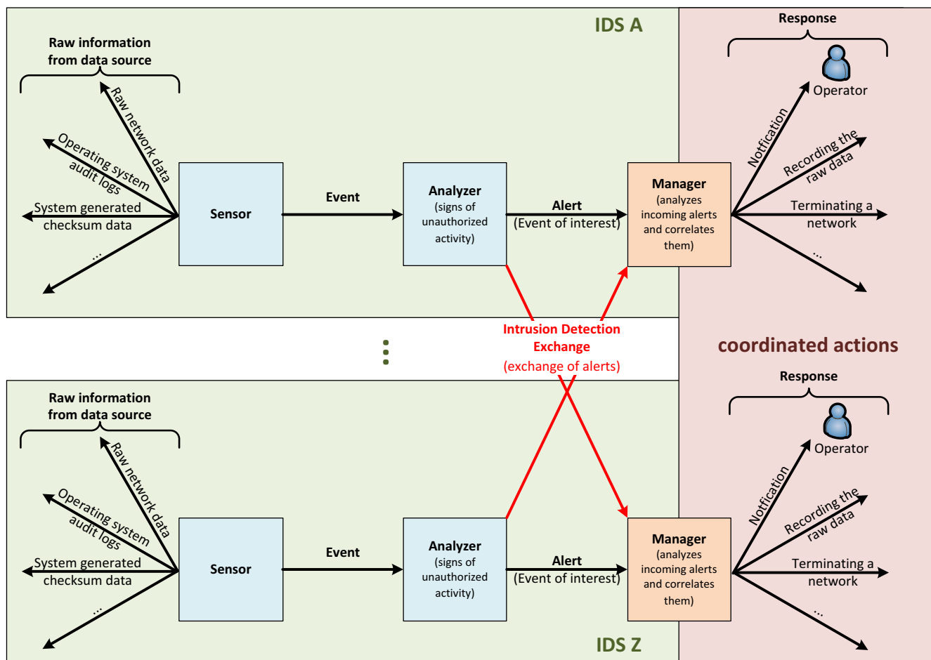
Fig. 3. Process of Information Exchange between IDSs
