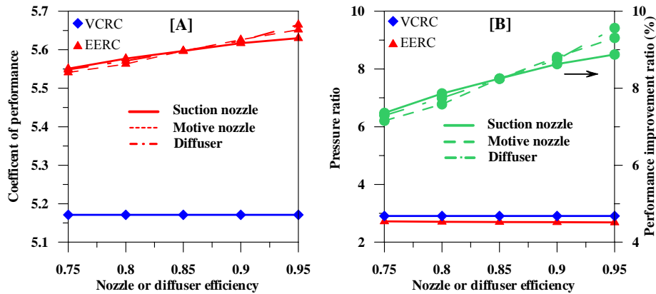
Fig. 7 Effect of nozzle and diffuser efficiencies on coefficient of performance, performance improvement ratio and pressure ratio
