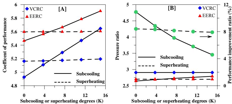
Fig. 8 Effect of subcooling and superheating degrees on coefficient of performance, performance improvement ratio and pressure ratio
