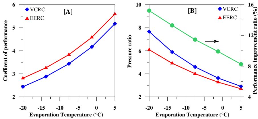
Fig. 6 Variation of coefficient of performance, performance improvement ratio and pressure ratio with evaporation temperature
