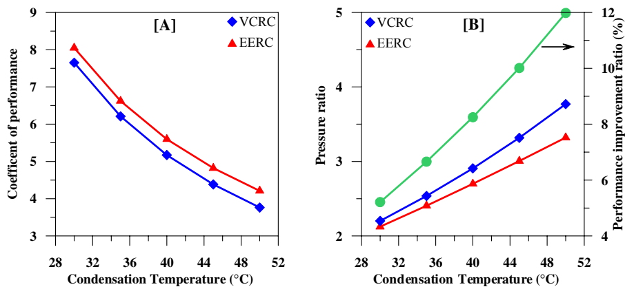
Fig. 5 Variation of coefficient of performance, performance improvement ratio and pressure ratio with condensation temperature
