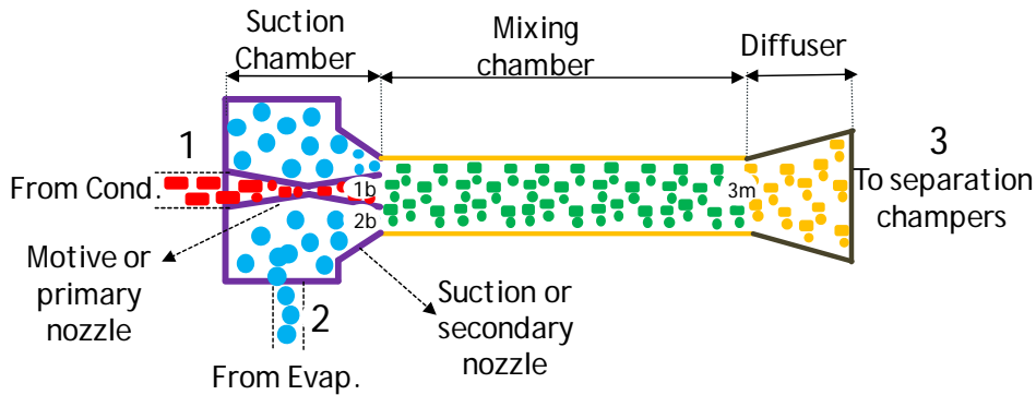
Fig. 2 Schematic diagram of constant area ejector flow model
