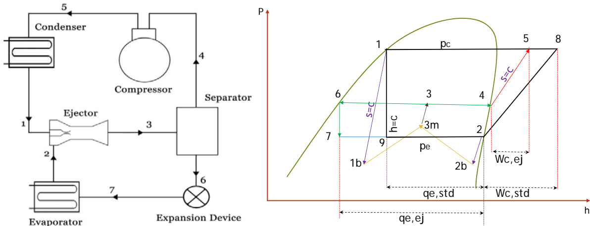
Fig. 1 Schematic diagram of ejector expansion refrigeration cycle and p-h diagram
