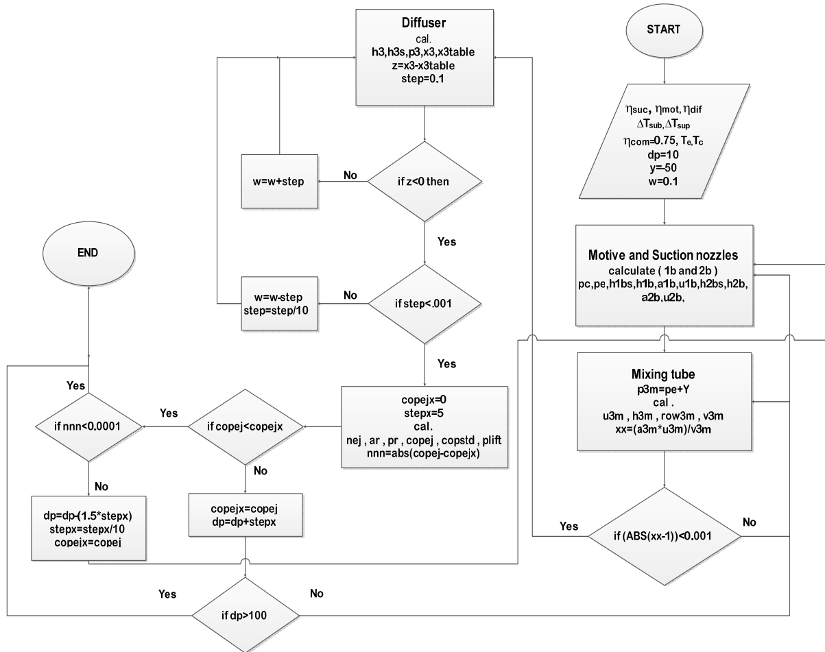
Fig. 3 Flow chart of the simulation program
