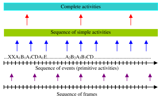
Fig. 6 Hierarchal approach for recognizing medication intake.
