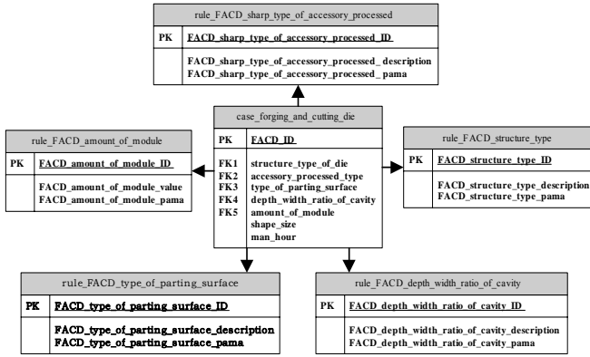
Fig. 4 The E-R diagram of the instance
