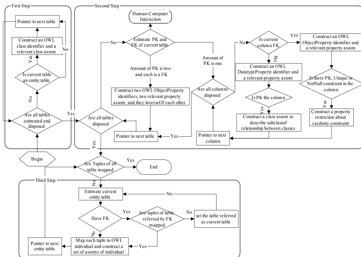
Fig. 3 The Flow of Automatic Mapping Algorithm
