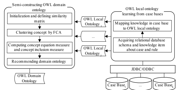
Fig. 2 The semi-automatic construction approach flow
