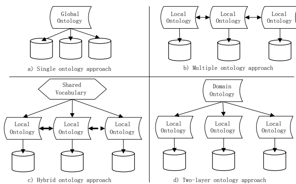
Fig. 1 Architecture of ontology-based integration approach
