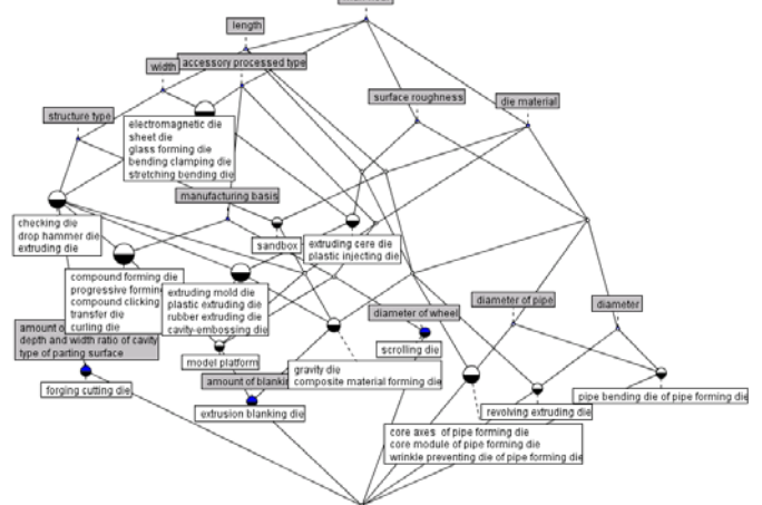
Fig. 7 The Hasse diagram of concept lattice instance
