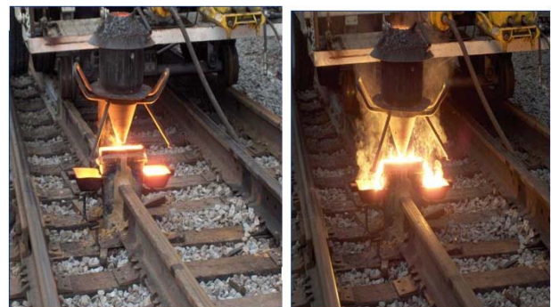
Fig.1 Thermite welding
