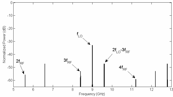
Fig.2. The generated electrical signal with \phi_o = \pi / 2
