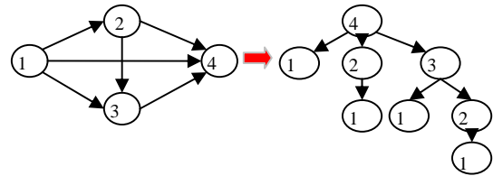
Fig. 1 An example of ETS transformation
