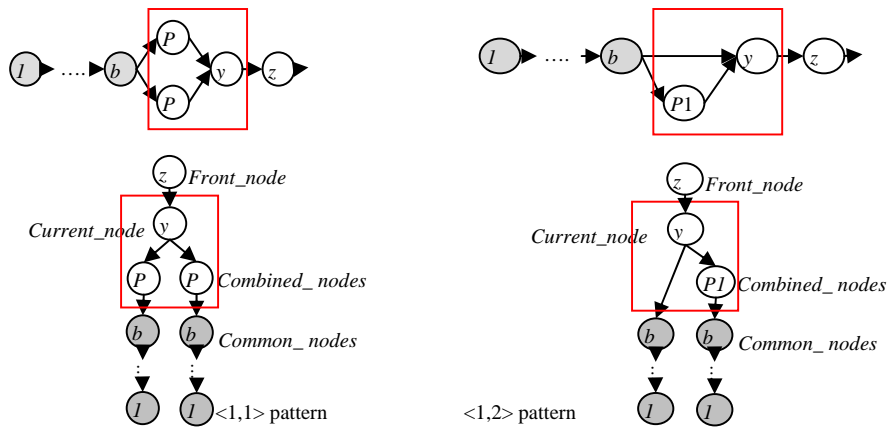
Fig. 3 <1,1> and <1,2> structure patterns of Parallel combination
