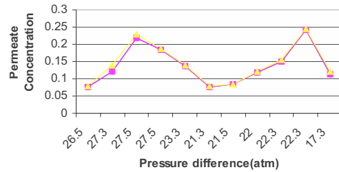
Fig. 2 Comparison of permeate concentration from numerical and experimental
