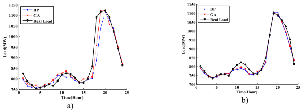
Fig. 11. ANN forecasted loads for sample of two special days: (a) Gorban festival (b) 22 Bahman.
