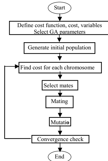
Fig.7. Flowchart of a continuous GA
