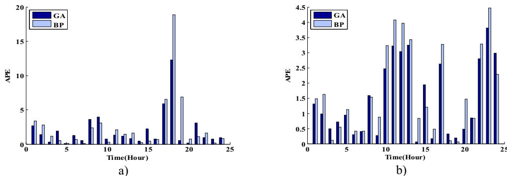
Fig.12. APE of two typical of special days: (a) Gorban festival (b) 22 Bahman.
