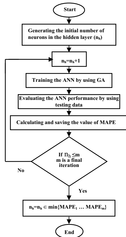
Fig. 4. The flowchart of the proposed method
