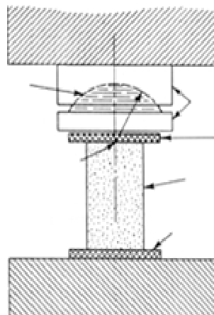
Fig. 6. Crushing Strength Tester [5]
