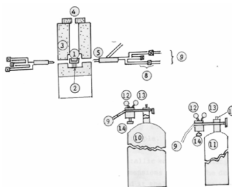
Fig. 2. Arrangement of Test Cones
