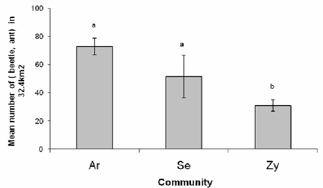
Fig. 1 Mean ± SE number of ants and beetles in each habitat.
