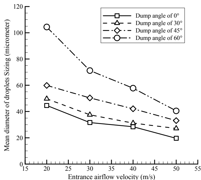
Fig. 3 The variation of mean diameter in different entrance airflow velocity
