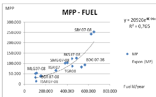
Fig. 4 Private Passenger Vehicle – Fuel Consumption of Metropolitan and Large Cities
