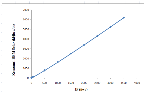
Fig. 11 Simulation on the Influence of Population in the Prediction of the Diesel Fuel Consumption of Metropolitan and Large Cities in Java
