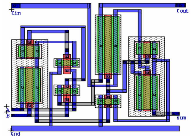
Fig. 8 Layout of the proposed 8T full adder
