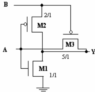
Fig. 3 Design of 3T XOR gate
