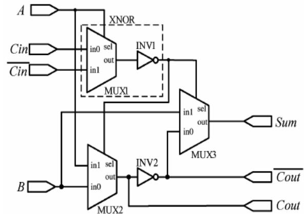
Fig. 2 Logic block diagram of CLRCL full adder.
