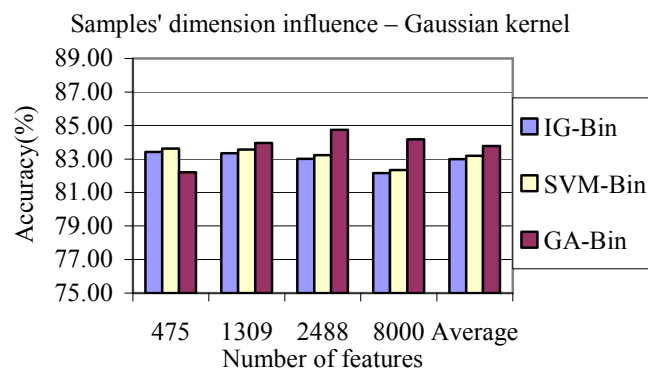
Fig. 4 Influence of the number of features on the classification accuracy using Gaussian kernel with parameter C equal to 1.3
