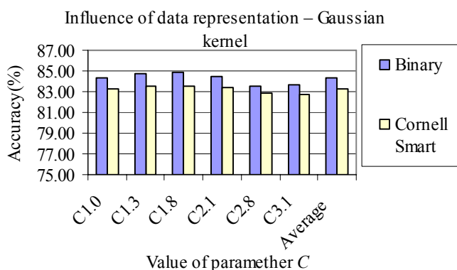
Fig. 2 Influence of data representation and parameter C for Gaussian kernel
