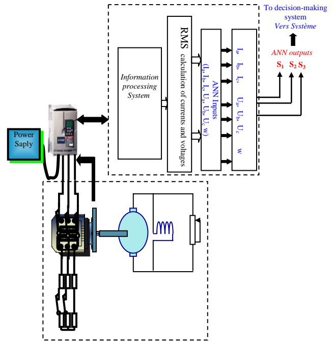
Fig. 4 Development of the defect automatic diagnosis system architecture of the asynchronous machine for an experimental realization
