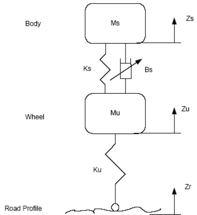
Fig. 3 Two DOF suspension model
