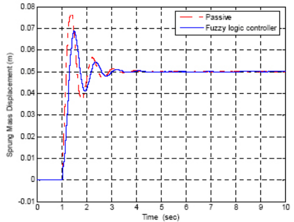
Fig. 7 Comparison of the responses of passive and semi active suspension systems to a step input
