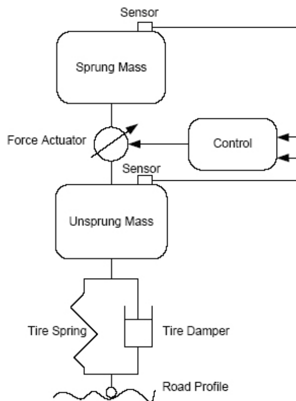
Fig. 1 Schematic of an active suspension system
