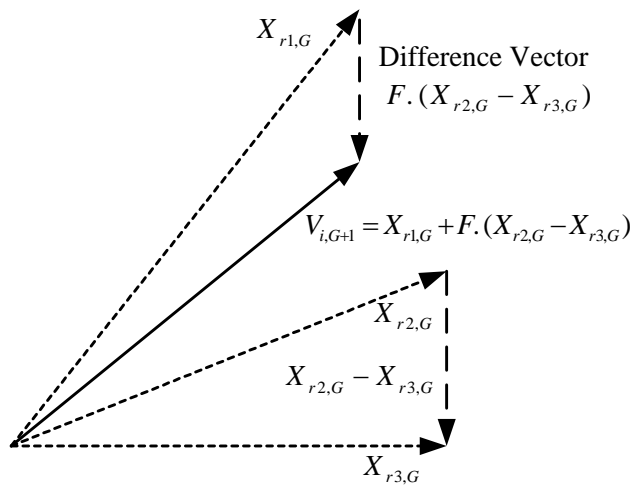
Fig. 3 Vector addition and subtraction in differential evolution
