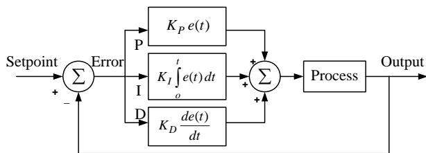
Fig. 2. Structure of PID controller
