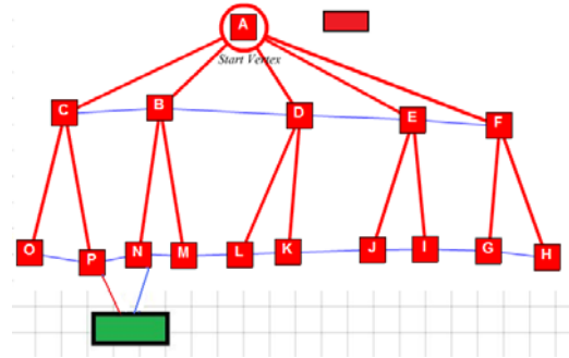
Fig. 4 BFS spanning tree for master node A
