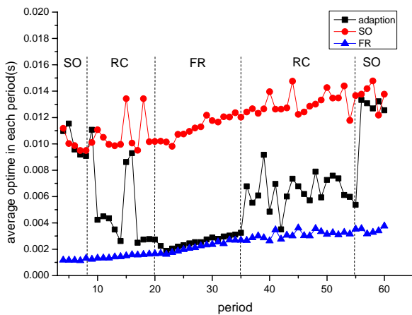
Fig. 5 Read operation executing time along periods
