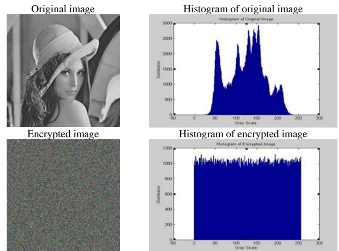
Fig. 7 Histograms of the Plainimage and the cipherimage
