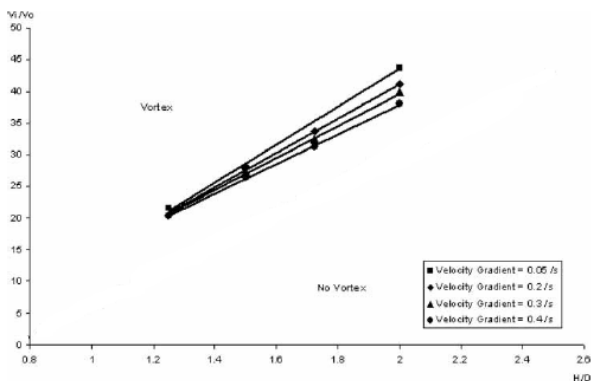
Fig. 2 Vortex formation threshold from computational studies [6]
