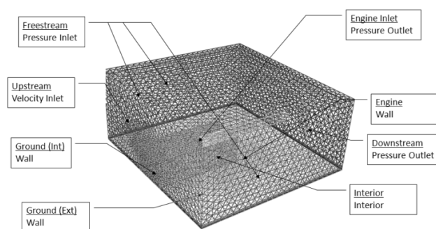
Fig. 5 Boundary Conditions
