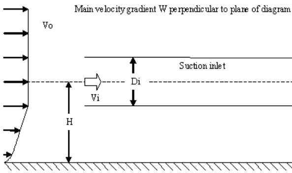
Fig. 1 Sketch showing the principal parameters
