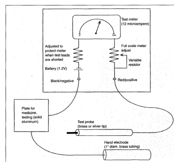
Fig. 3 A simple schematic diagram of an EDSD
