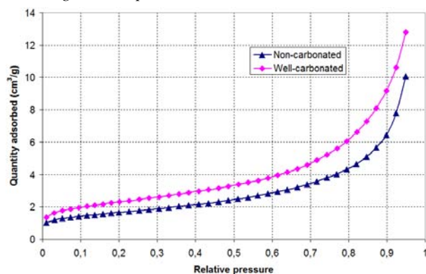
Fig. 1 Nitrogen adsorption isotherms of cement mortar
