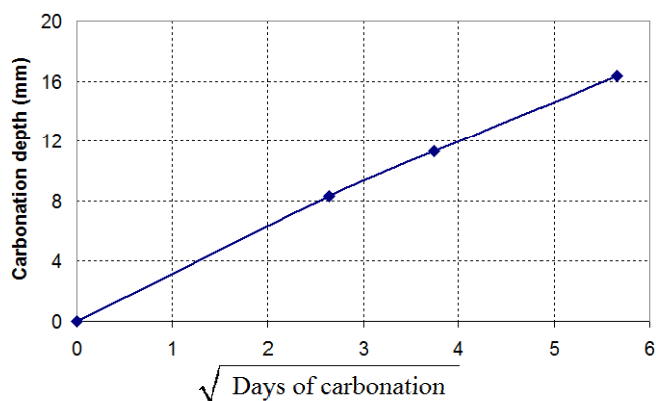
Fig. 4 Evolution of the carbonation depth during carbonation
