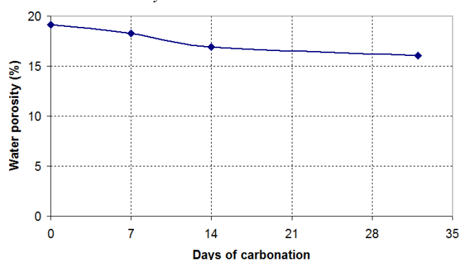
Fig. 5 Evolution of the porosity accessible to water during carbonation
