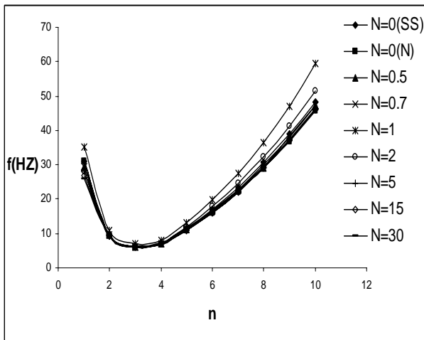
Fig. 2 Natural frequencies FG cylindrical shell associated with various power law exponent for F-F boundary condition.
