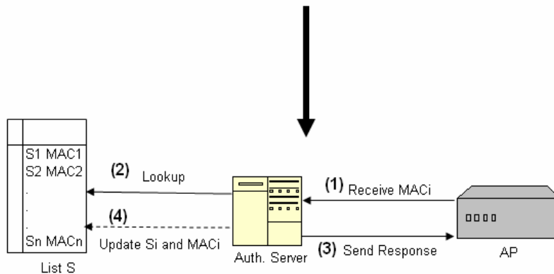
(a) Traditional MAC Address Authentication
