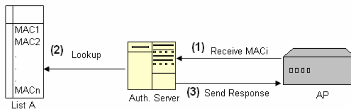
(a) Traditional MAC Address Authentication
