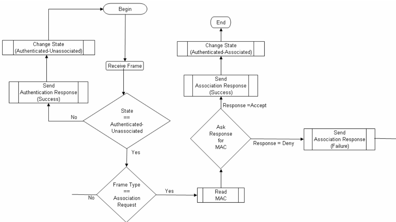
Fig. 3 Operation of MAC authentication in Mode 1
