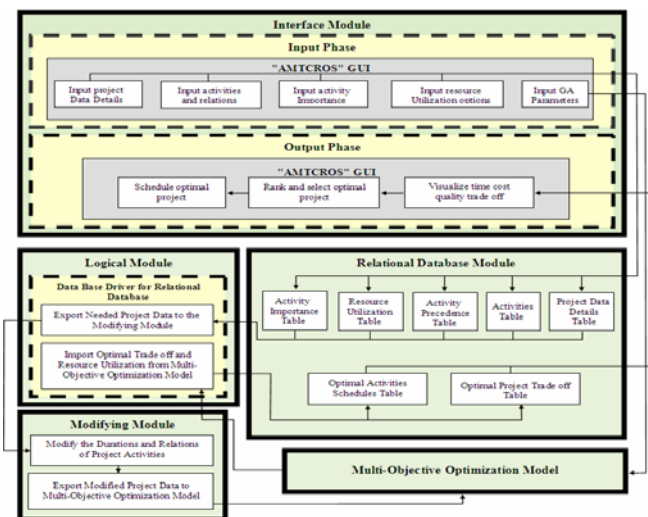
Fig. 2 The Main Modules of "AMTCROS" System
