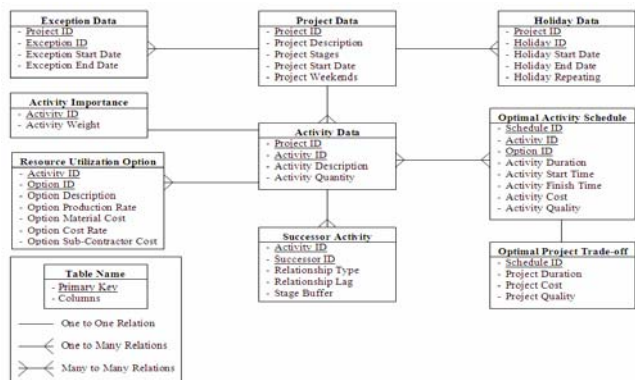
Fig. 3 Relational Database Design
