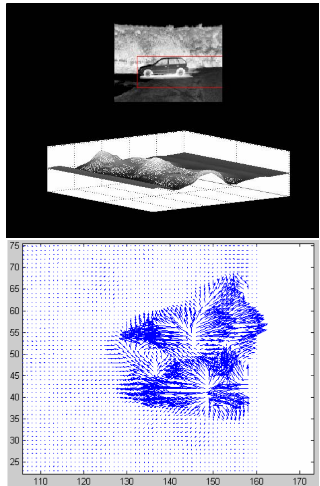
Fig. 3 Optical Flow and MACH filter results on the target for a video frame filmed with a stationary camera
