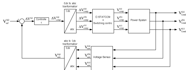
Fig. 3 Complete block diagram of voltage regulation scheme
