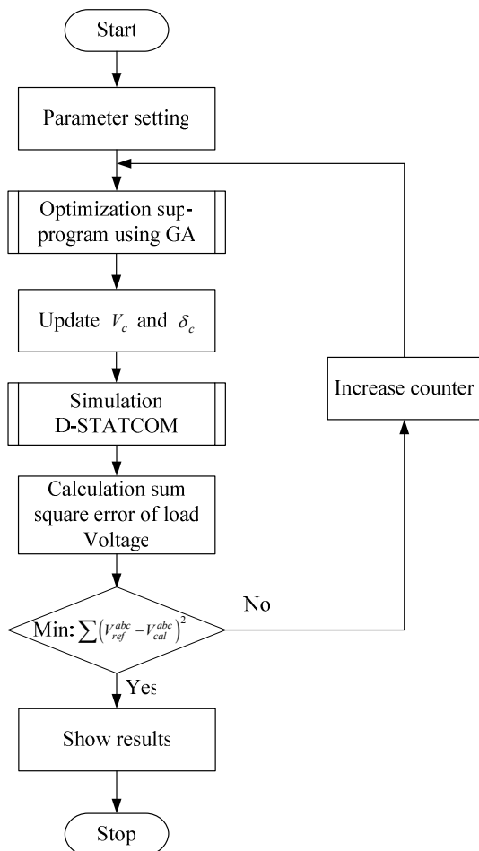
Fig. 5 Flow chart of the genetic algorithm
