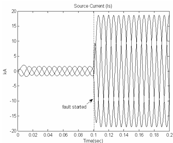
Fig. 9 Source currents of the base case
