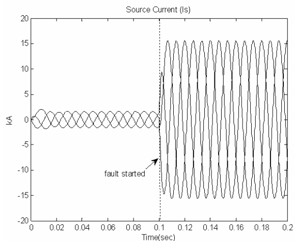
Fig. 12 Source currents of the D-STATCOM case
