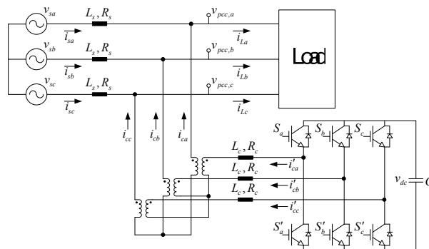
Fig. 1 Circuit structure of D-STATCOM
