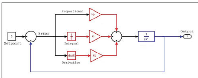
Fig. 16. Block diagram of the PID Controller
