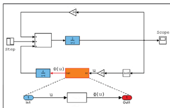
Fig. 20. Block-diagrams of the Nonlinear accelerator
