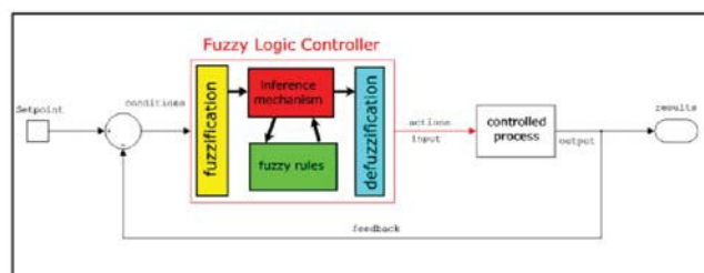
Fig. 1. Design the fuzzy controller
