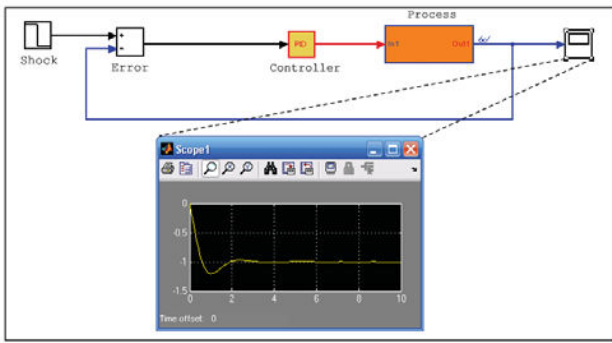
Fig. 15. Block diagram of the closed-loop system
