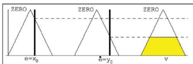
Fig. 6. FAM influence procedure with crisp input measurements
