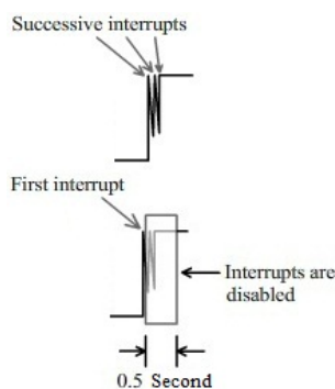
Fig. 6 De-bouncing
