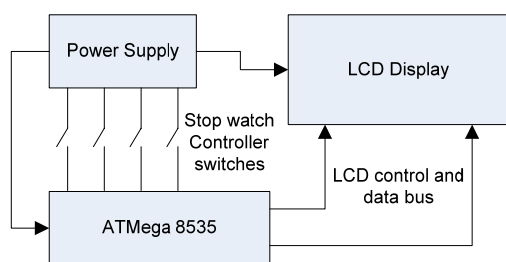
Fig. 1 Block diagram of the stop watch system
