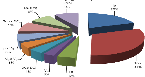
Fig. 4 Percentage contribution of the factors for out of roundness in EDM with cryogenically cooled electrode
