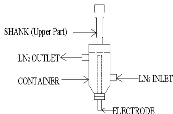
Fig. 1 The schematic diagram of electrode attachment [14]
