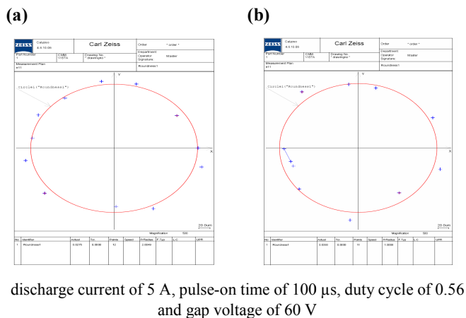
Fig. 2 Graphs showing the values of out of roundness for the electrode at same processing conditions (a) with cryogenic assistance (b) without cryogenic assistance
