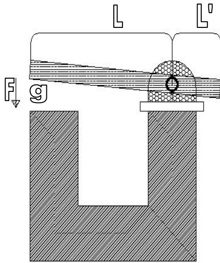
Fig. 7 Structure of electrical relay of EMABS
