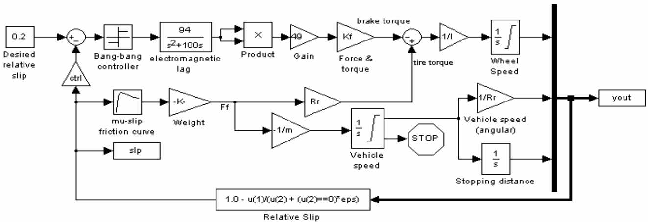
Fig. 15 EMABS SIMULINK block diagram
