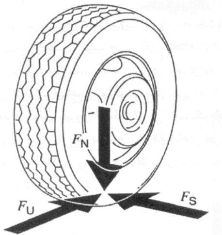
Fig. 3 Side, Longitudinal and Normal forces on tire
