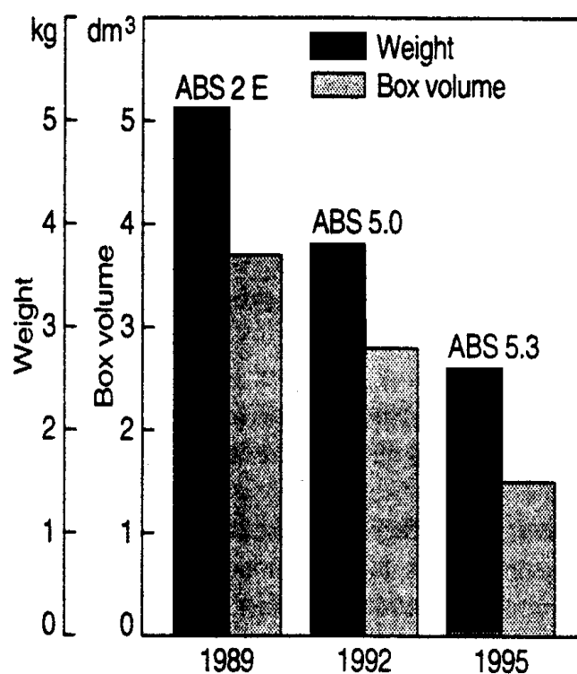
Fig. 1 Evolution of ABS system in time
