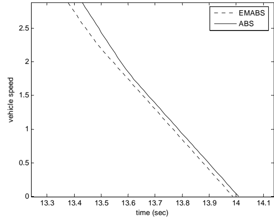
Fig. 10 comparing vehicle speed with ABS and EMABS .
