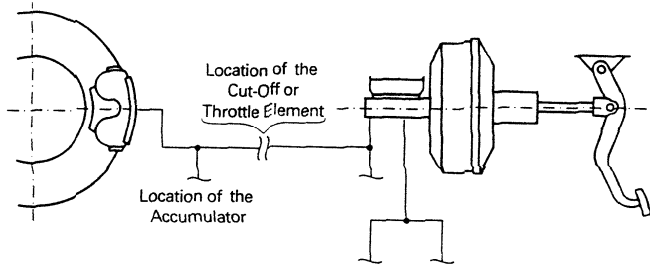
Fig. 2 Overall configuration of the hydraulic brakes
