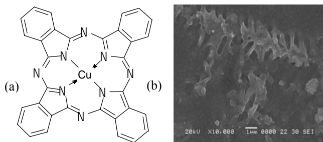
Fig. 1 (a) Molecular structure of copper phthalocyanine (CuPc). (b) SEM image of the CuPc film.
