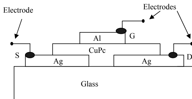
Fig. 2 Cross sectional view of the organic FET
