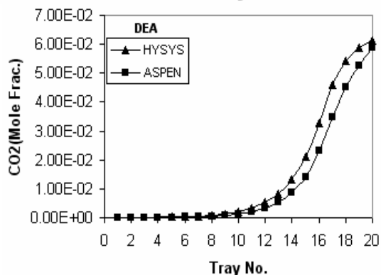
Fig. 4 Stage number vs. CO 2 and H 2 S vapor composition profiles in the absorber
