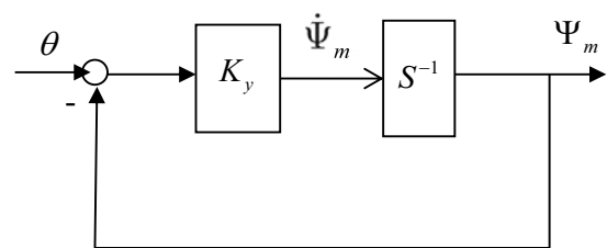
Fig. 4 Feedback linearization control diagram
