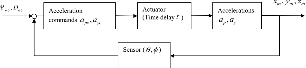
Fig. 5 Missile acceleration command working diagram
