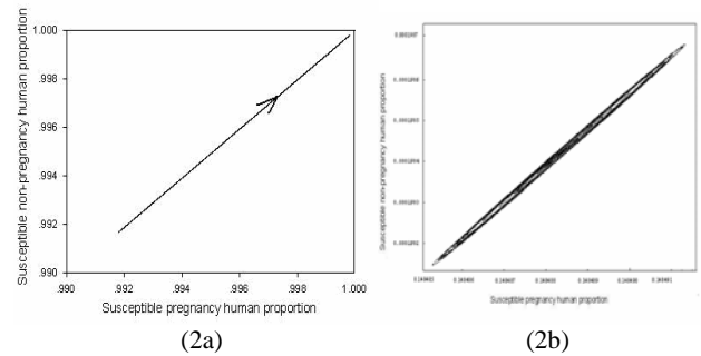
Fig. 2 Numerical solutions of (3), demonstrate the solution trajectories, projected onto (S^p, S^n)
