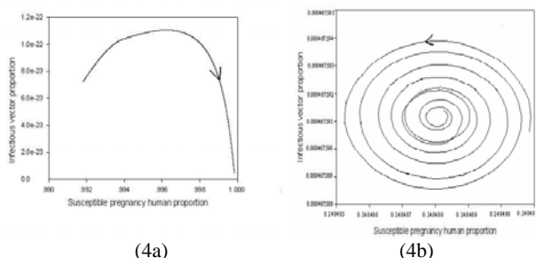
Fig. 4 Numerical solutions of (3), demonstrate the solution trajectories, projected onto (S^p, I^v)
