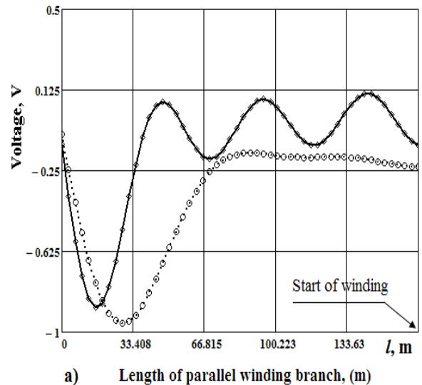
Fig. 3 Wave process in the winding phase of the motor — Applied impulsion on the phase — Tension on the first section of the winding - - - Tension on the last section of the winding a) a = 1; b) a = 2
