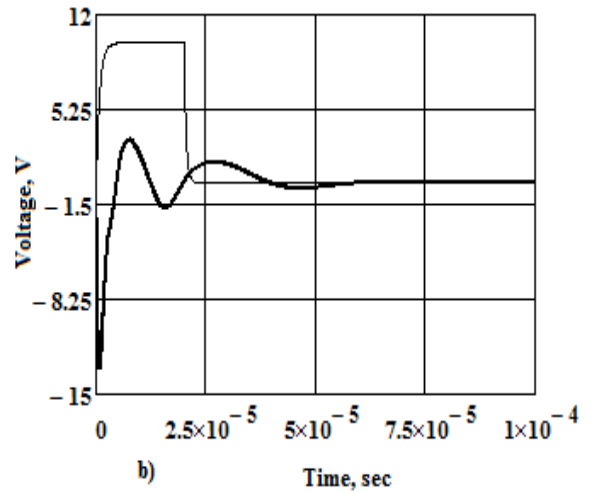
Fig. 3 Wave process in the winding phase of the motor — Applied impulsion on the phase — Tension on the first section of the winding - - - Tension on the last section of the winding a) a = 1; b) a = 2
