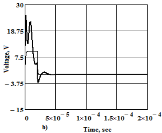
Fig. 3 Wave process in the winding phase of the motor — Applied impulsion in the winding — Applied impulsion in the winding a) a = 1; b) a = 2
