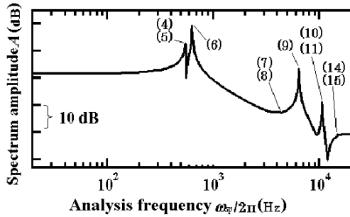
Fig. 5 Fourier spectrum of impact response under small input
