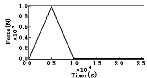
Fig. 4 Small input of impact load
