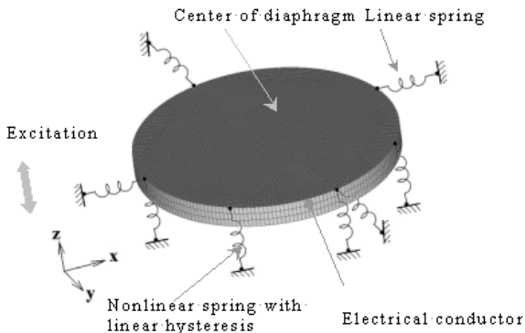
Fig. 1 Simulation model
