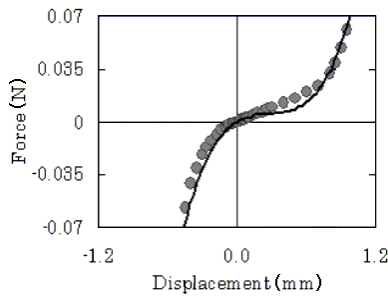
Fig. 2 Restoring force of nonlinear concentrated springs (●: Experiment —: Approximation)
