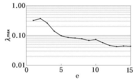
Fig. 7 Largest Lyapunov exponent against embedded dimension
