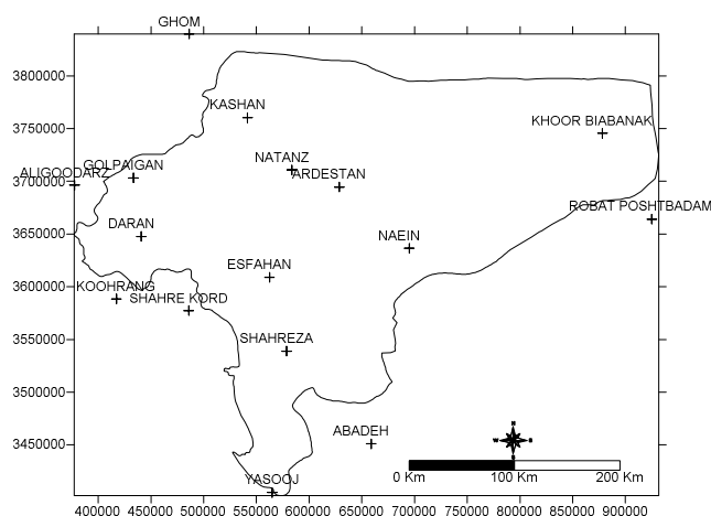
Fig. 1 Location of synoptical stations in Isfahan province
