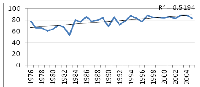
Fig. 7 The time series of September tci index in Isfahan province
