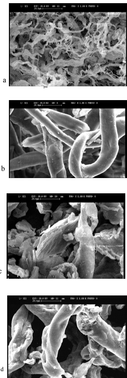
Fig. 3 SEM images of (a) BC, (b) cellulose, (c) CMBC and (d) standard CMC.
