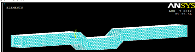
Fig. 5 Mesh model of Catalyst with tortuous path
