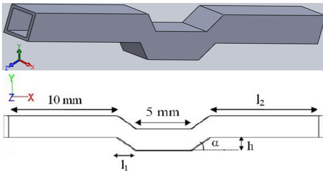
Fig. 3 Design of Catalyst with tortuous path
