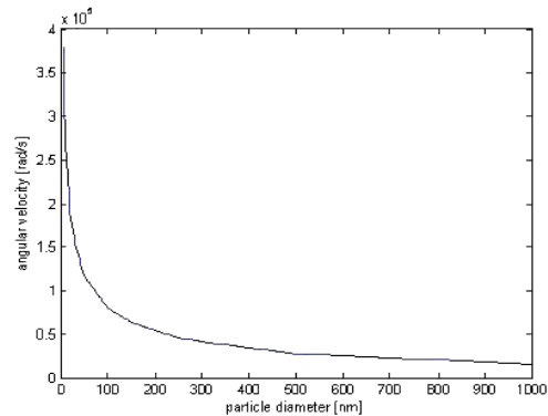
Fig. 7 Particle movements in a Vortex
