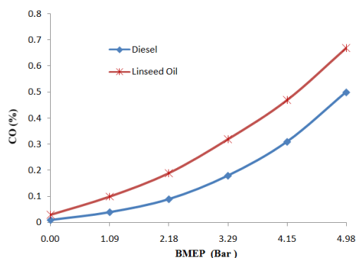
Fig. 6 Variation of carbon mono oxide with brake means effective pressure
