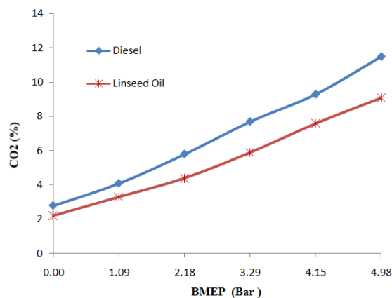
Fig. 7 Variation of carbon di oxide with brake means effective pressure
