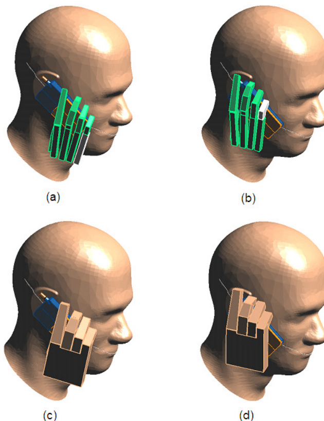
Fig. 3 Different CAD representations of the handset in hand close to head at cheek-position; (a) Hand1-bones holding the handset, (b) Hand2-bones holding the handset, (c) Hand1-tissues holding the handset and (d) Hand2-tissues holding the handset.
