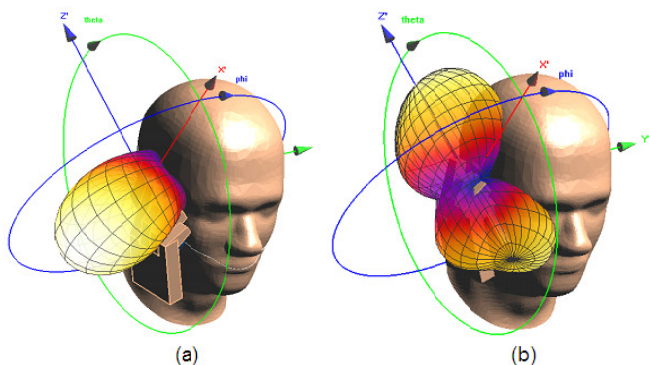
Fig. 6 The 3-D far-field radiation pattern; (a) handset in hand1 close to SAM at cheek-position and (b) handset in hand2 close to SAM at cheek-position..
