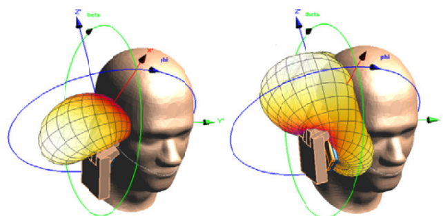
Fig. 7 The 3-D far-field radiation pattern; (a) handset in hand1 close to SAM at tilt-position and (b) handset in hand2 close to SAM at tilt-position.
