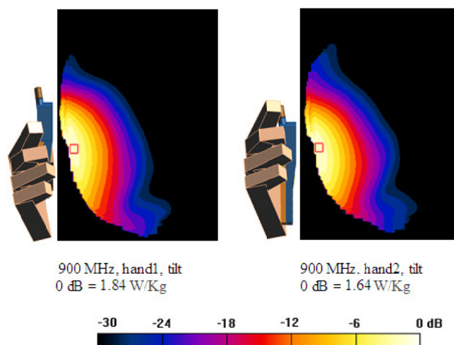
Fig. 9 The peak SAR 1g sliced-distribution (yz- plane) in SAM due to the EM radiation of the handset antenna at tilt-position.
