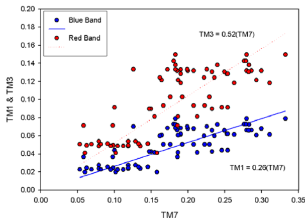
Fig. 2 Correlation between visible and mid infrared surface reflectances for Landsat TM
