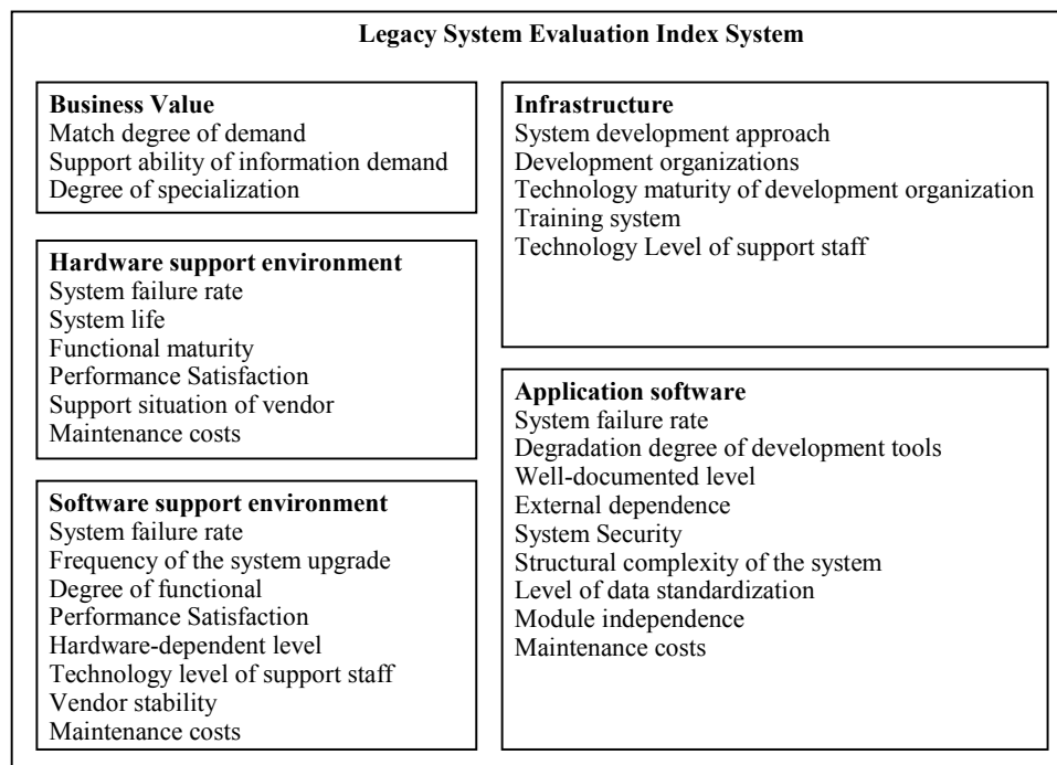
Fig. 1 Legacy System Evaluation Index System
